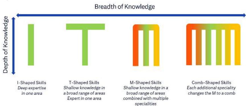
Figure 17. Skills Shapes
